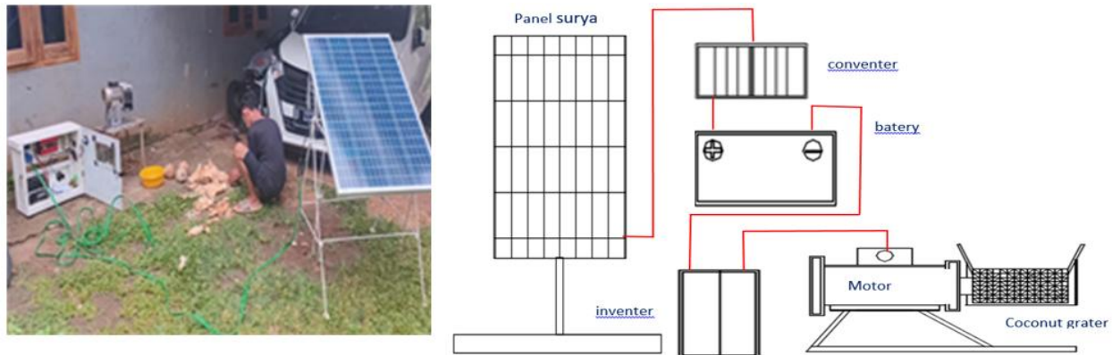
Figure 1. Solar-powered coconut grating machine circuit
