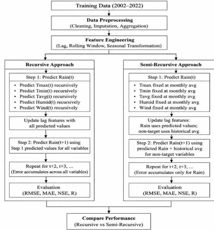
Figure 2. Research flowchart
